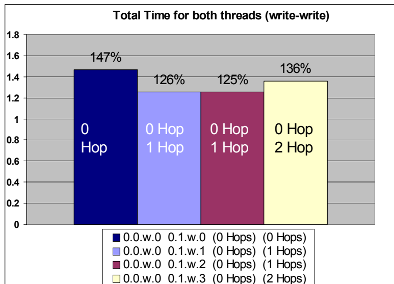
Figure 11. Both Write-Only Threads Running on Node 0 (Different Cores) on an Idle System
