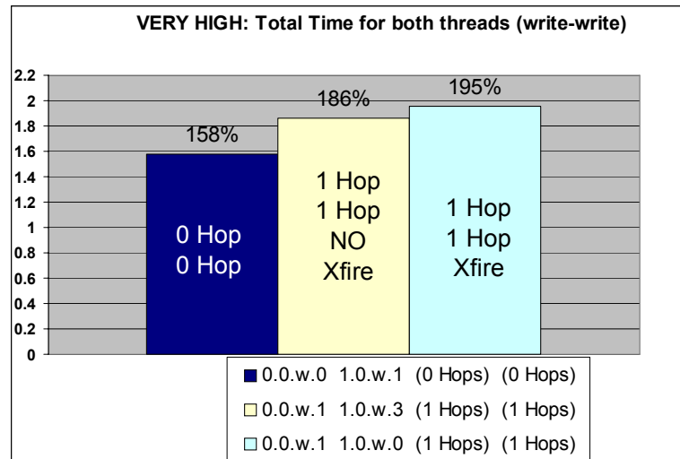
Figure 8. Crossfire 1 Hop-1 Hop Case vs No Crossfire 1 Hop-1 Hop Case under a Very High Background Load (High Subscription)
