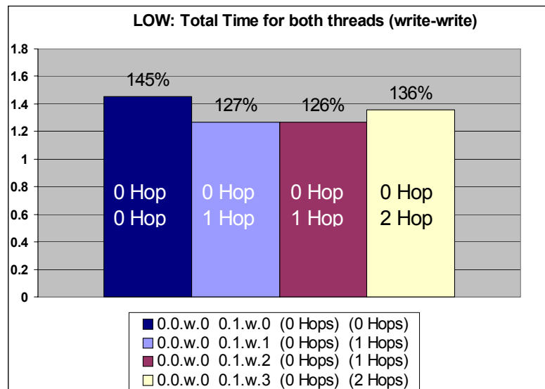
Figure 12. Both Write-Only Threads Running on Node 0 (Different Cores) under Low Background Load (High Subscription)
