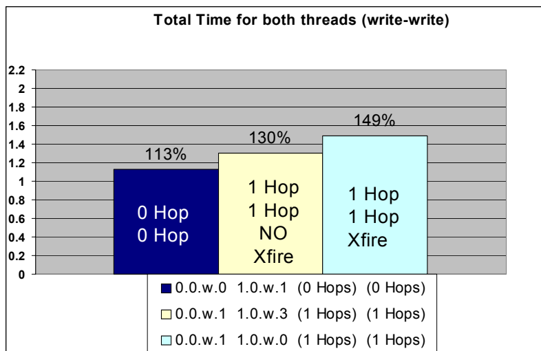
Figure 6. Crossfire 1 Hop-1 Hop Case vs No Crossfire 1 Hop-1 Hop Case on an Idle System
