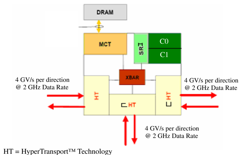
Figure 2. Internal Resources Associated with a Quartet Node
