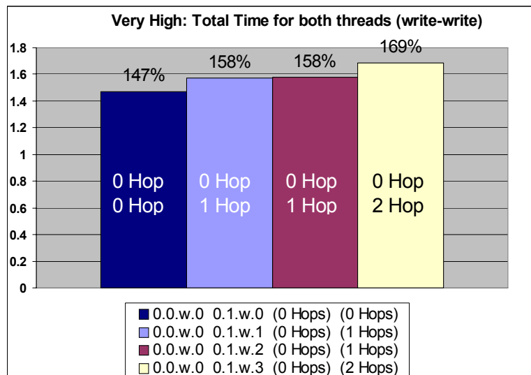
Figure 15. Both Write-Only Threads Running on Node 0 (Different Cores) under Very High Background Load (High Subscription)
