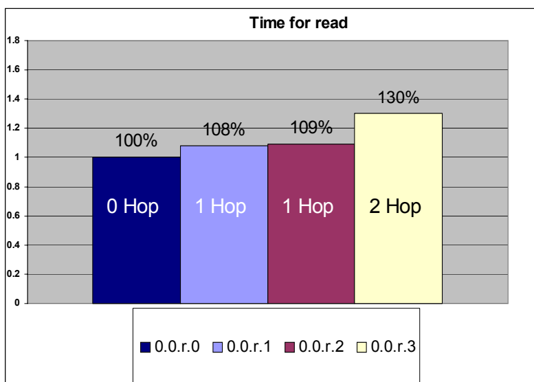
Figure 4. Read-Only Thread Running on Node 0, Accessing Data from 0, 1 and 2 Hops Away on an Idle System
