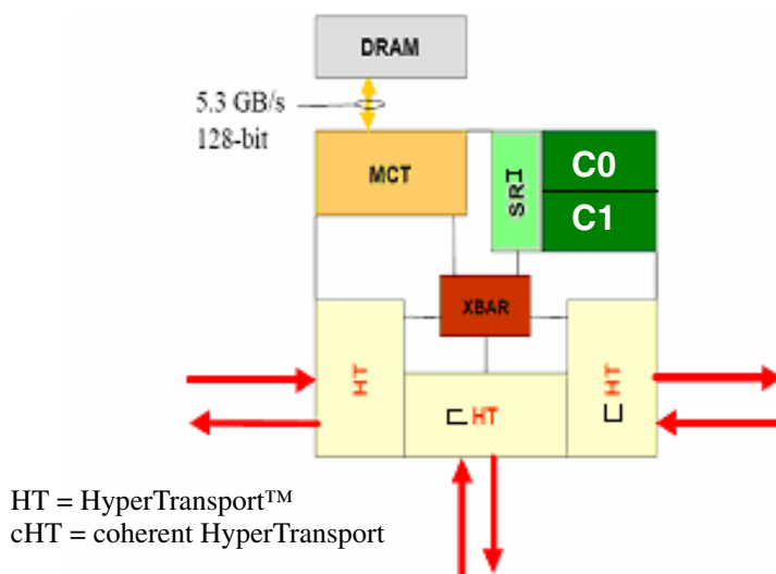
Figure 16. Internal Resources Associated with a Quartet Node
