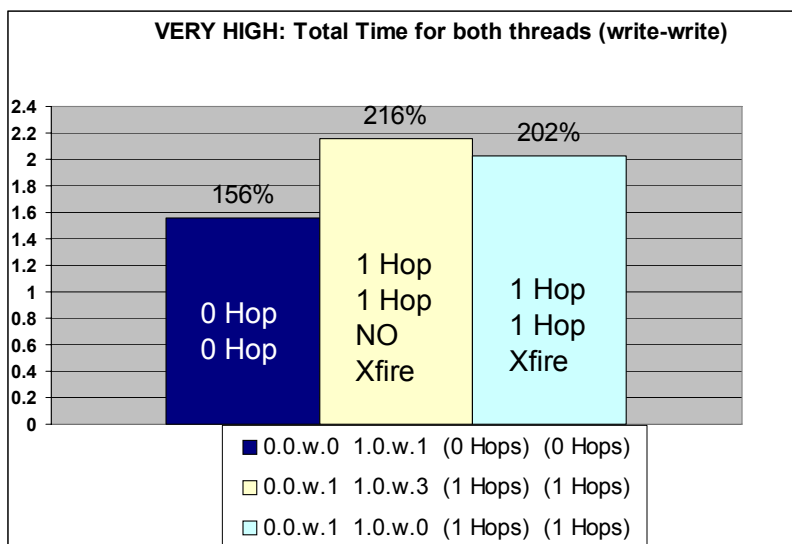
Figure 9. Crossfire 1 Hop-1 Hop Case vs No Crossfire 1 Hop-1 Hop Case under a Very High Background Load (Full Subscription)
