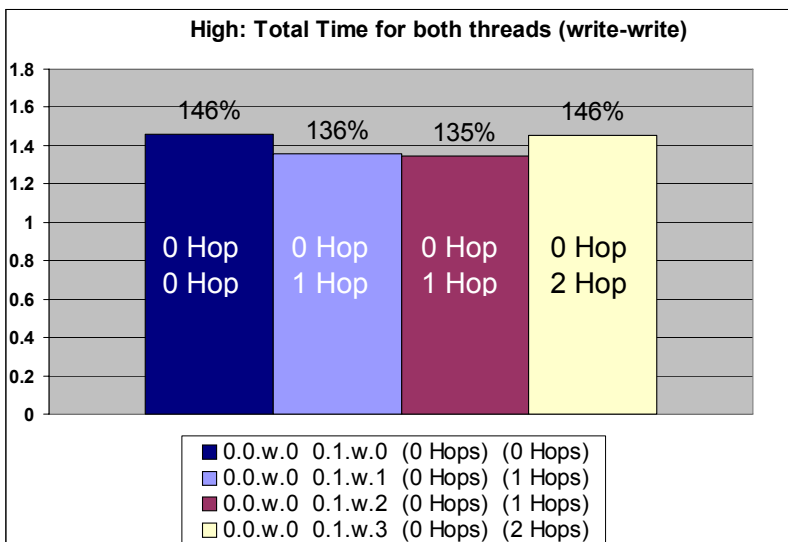
Figure 14. Both Write-Only Threads Running on Node 0 (Different Cores) under High Background Load (High Subscription)
