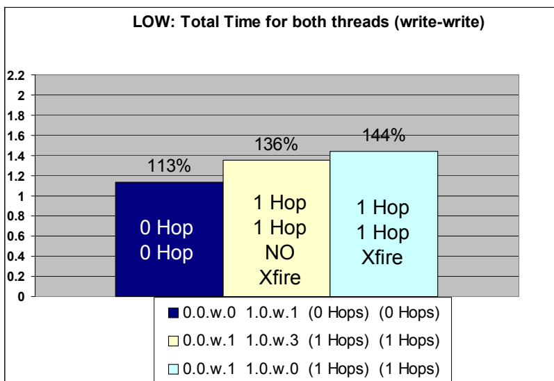
Figure 7. Crossfire 1 Hop-1 Hop Case vs No Crossfire 1 Hop-1 Hop Case under a Low Background Load (High Subscription)
