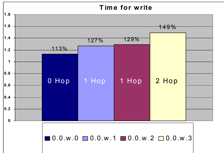
Figure 5. Write-Only Thread Running on Node 0, Accessing Data from 0, 1 and 2 Hops Away on an Idle System
